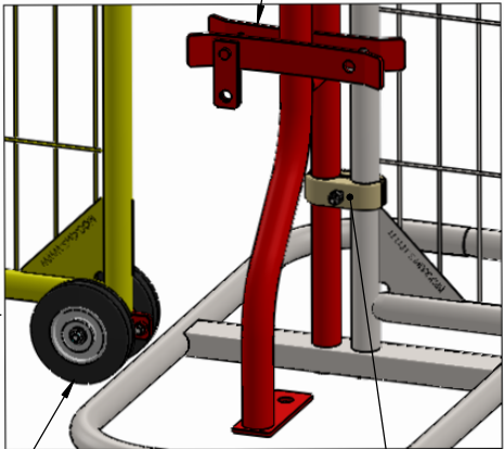
WHEEL CLAMP ASSEMBLY 08051541-3
